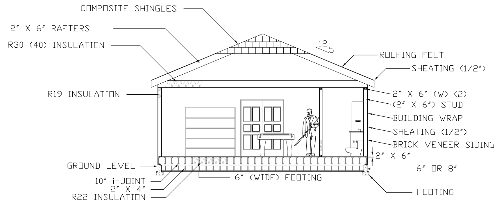
CROSS SECTION SCALE 1/8" = 1'
