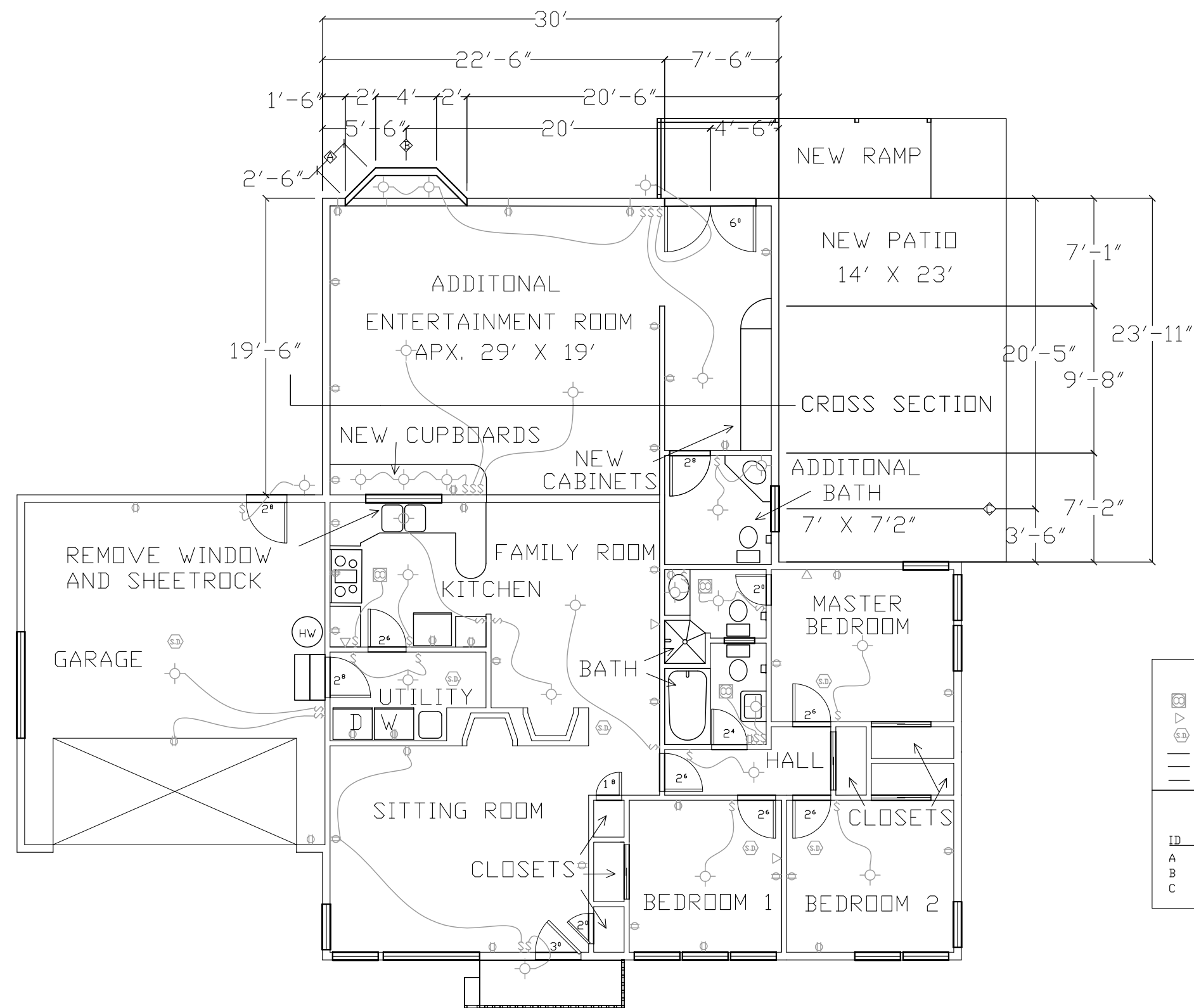
FLOOR PLAN SCALE 1/8" = 1' NORTH
